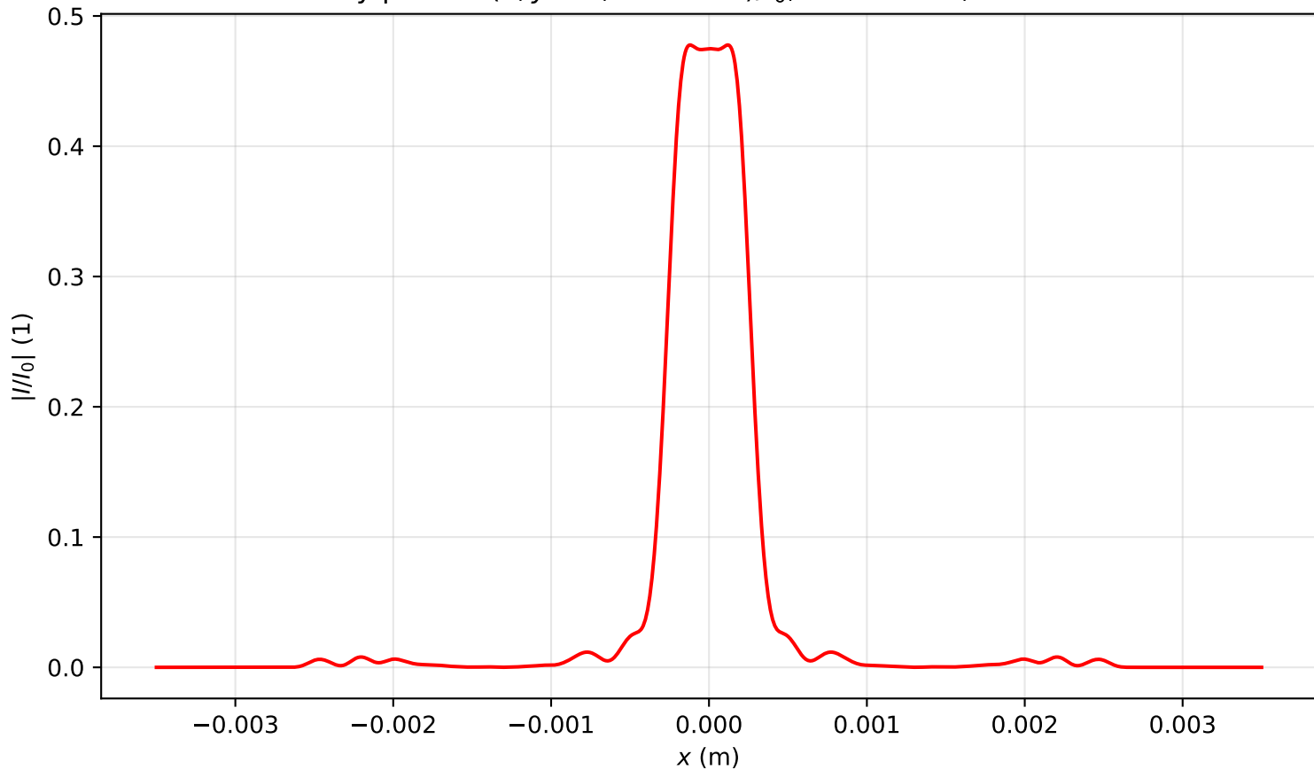
Intensity profile I(x, y = 0, z = 1.592)/I_0 , P_{in}=5.0P_{cr} , artificial time
